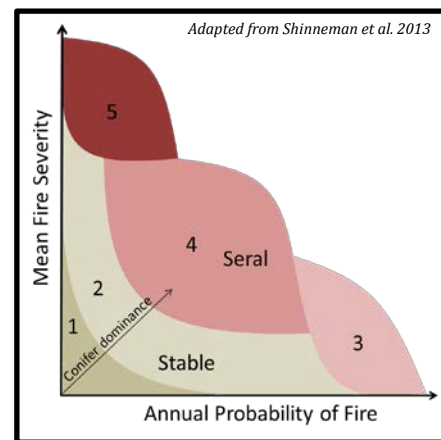
Fig. 2. Five aspen fire-regime types in two dimensional “fire space”
